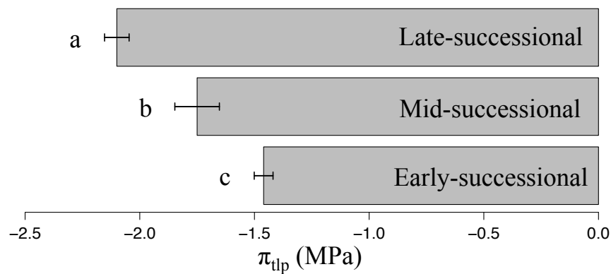
Figure 3: Differences in leaf water potential at wilting point ( \pi_{tlp} , in MPa) across successional stages, for early-, mid- and late-successional canopy trees ( n=11 , 10 and 29 individuals respectively). Means \pm standard errors are reported. Different lower case letters indicate a significant difference between stages (Tukey test: P < 0.05 ).
