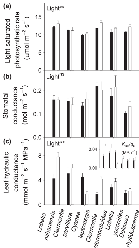
Fig. 2 Plastic response of physiological traits in response to growth irradiance for six ecologically diverse species of Hawaiian lobeliads. Mean \pm SE values for light-saturated \text{CO}_2 assimilation rate ( A_{\text{max}} ) (a), stomatal conductance ( g_s ) (b), and leaf hydraulic conductance ( K_{\text{leaf}} ) (c) under low irradiance (closed bars) and high irradiance (open bars). The inset in (c) shows hydraulic supply over demand ( K_{\text{leaf}}/g_s ) under low irradiance (closed bars) and high irradiance (open bars). All traits showed significant variation across species ( P < 0.01 , ANOVA, Table 2: ^{ns} , P > 0.05 ; ^{**} , P < 0.01 ).
