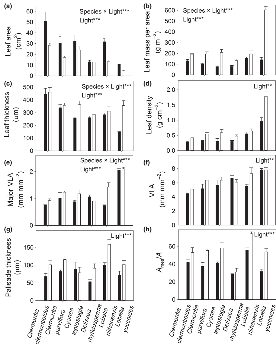
Fig. 4 Plastic response of anatomical and structural traits to growth for six ecologically diverse species of Hawaiian lobeliads. Mean \pm SE values for leaf area (a), leaf mass per area (LMA) (b), leaf thickness (c), leaf density (d), major vein length per area (major VLA) (e), total vein length per area (VLA) (f), palisade tissue thickness (g), and mesophyll surface area per leaf area ( A_{\text{mes}}/A ) (h) for individuals grown under low irradiance (closed bars) and high irradiance (open bars). All these traits varied significantly across species ( P < 0.01 ; ANOVA, Table 2: **, P < 0.01 ; ***, P < 0.001 ).
