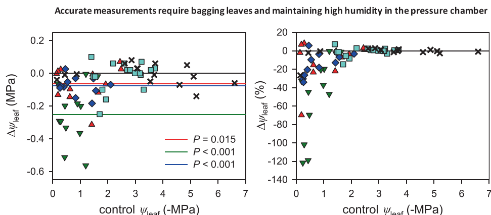
FIGURE 5 Assumption 5, i.e., accurate measurements require high humidity and bagged leaf in the chamber, tested on E. erythrocorys (▲), H. arbutifolia (▼), M. grandiflora (◆), C. cunninghamiana (■), and E. obliqua (✱). Controls represent \psi_{\text{leaf}} measured with moisture and bagged inside the chamber, and \Delta\psi_{\text{leaf}} is the difference in \psi_{\text{leaf}} between leaves without bag and any moisture inside the chamber and control leaves (with a positive value indicating a less negative value for treatment than control). \Delta\psi_{\text{leaf}} over control \psi_{\text{leaf}} is presented in terms of absolute values (left panel) and % of difference respect to control \psi_{\text{leaf}} (right panel). The horizontal line indicates that a significant difference was found between tested and control leaves but the regression was not significant. Each point represents a pair of matched leaves, i.e., the difference in \psi_{\text{leaf}} between tested and control leaves [Color figure can be viewed at wileyonlinelibrary.com ]
