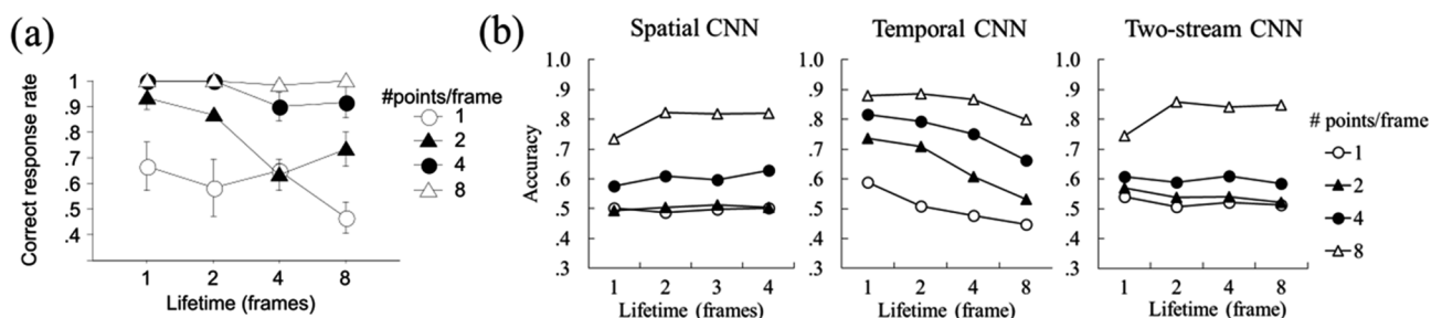
Fig. 5. Results of Simulation 3: Human and model performance for walking direction discrimination of SP walkers as a function of dot numbers and dot lifetime. (a) Human accuracy in walking direction discrimination ( Beintema & Lappe, 2002 , Experiment 2). Error bars represent \pm 1 SE. (b) Simulation results from the spatial CNN, temporal CNN, and two-stream CNN model with fusion network.
