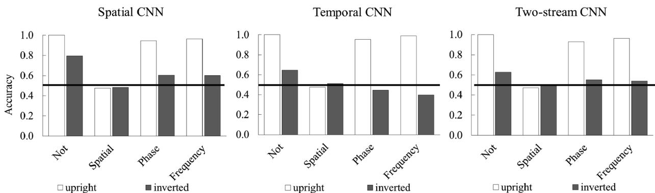
Fig. 6. Results of simulation 4: model performance for walking direction discrimination as a function of different scrambling conditions for upright and inverted walkers. Humans show an inversion effect in all four conditions ( Troje & Westhoff, 2006 ). All CNN models showed the inversion effect in intact, phase scrambling and frequency scrambling conditions, but neither model showed the inversion effect in spatial scrambled condition.
