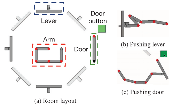
Figure 1: (a) Starting configuration of a 3-lever OpenLock room. The arm can interact with levers by either pushing outward or pulling inward, achieved by clicking either the outer or inner regions of the levers’ radial tracks, respectively. Light gray levers are always locked; however, this is unknown to agents. The door can be pushed only after being unlocked. The green button serves as the mechanism to push on the door. The black circle on the door indicates whether or not the door is unlocked; locked if present, unlocked if absent. (b) Pushing on a lever. (c) Opening the door.
