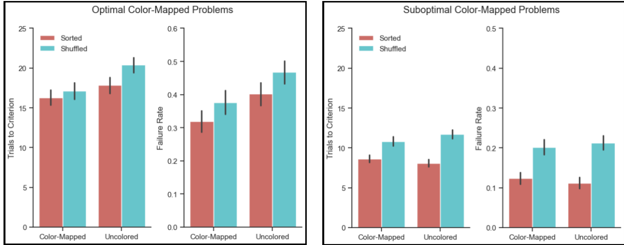
Figure 6. Trials-to-criterion and failure rates in Experiment 2 for optimal (left) and suboptimal (right) color-mapped problem sets. Error bars represent standard errors of the mean (trials-to-criterion) and binomial standard errors (failure rate) at the individual problem level.
